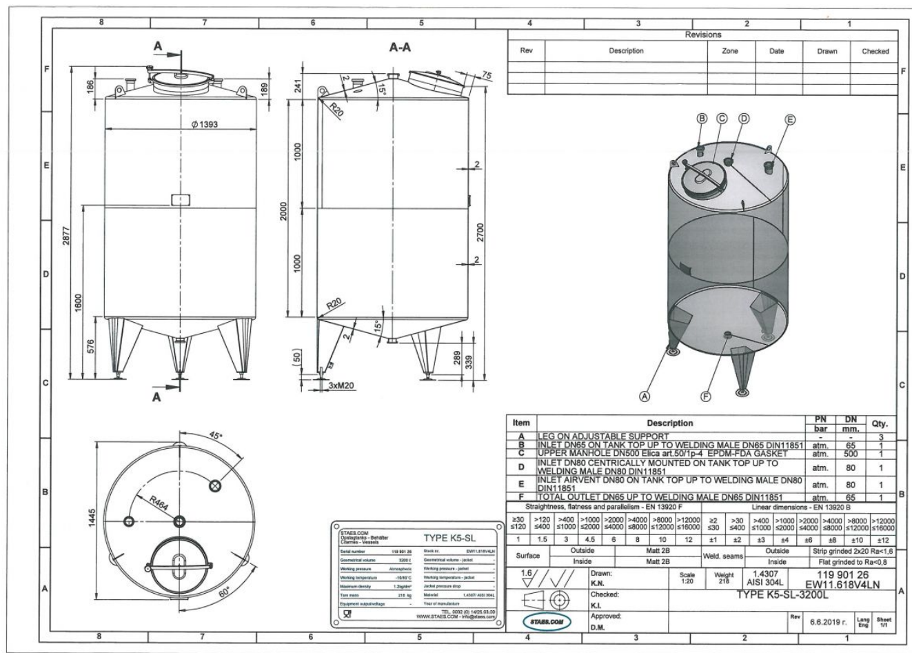
Technical drawing
